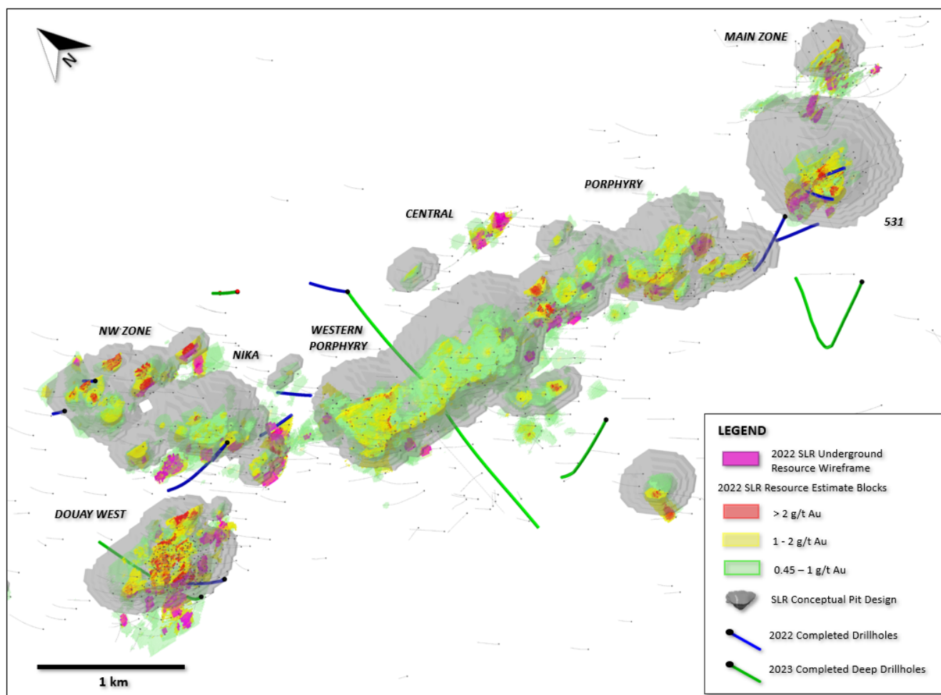
Figure 5: Douay oblique view showing pit-constrained resources at 0.45 g/t Au cut-off grade and underground resources at 1.15 g/t Au cut-off grade along with completed drilling since MRE (SLR 2022).
