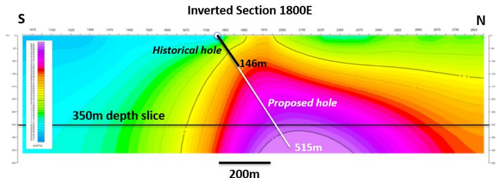
Inverted section shows significant broadening of high-contrast chargeability anomaly at depth; length of (projected) historical hole shown as black bar. White bar shows length of hole to be drilled in Fall 2020 campaign.
