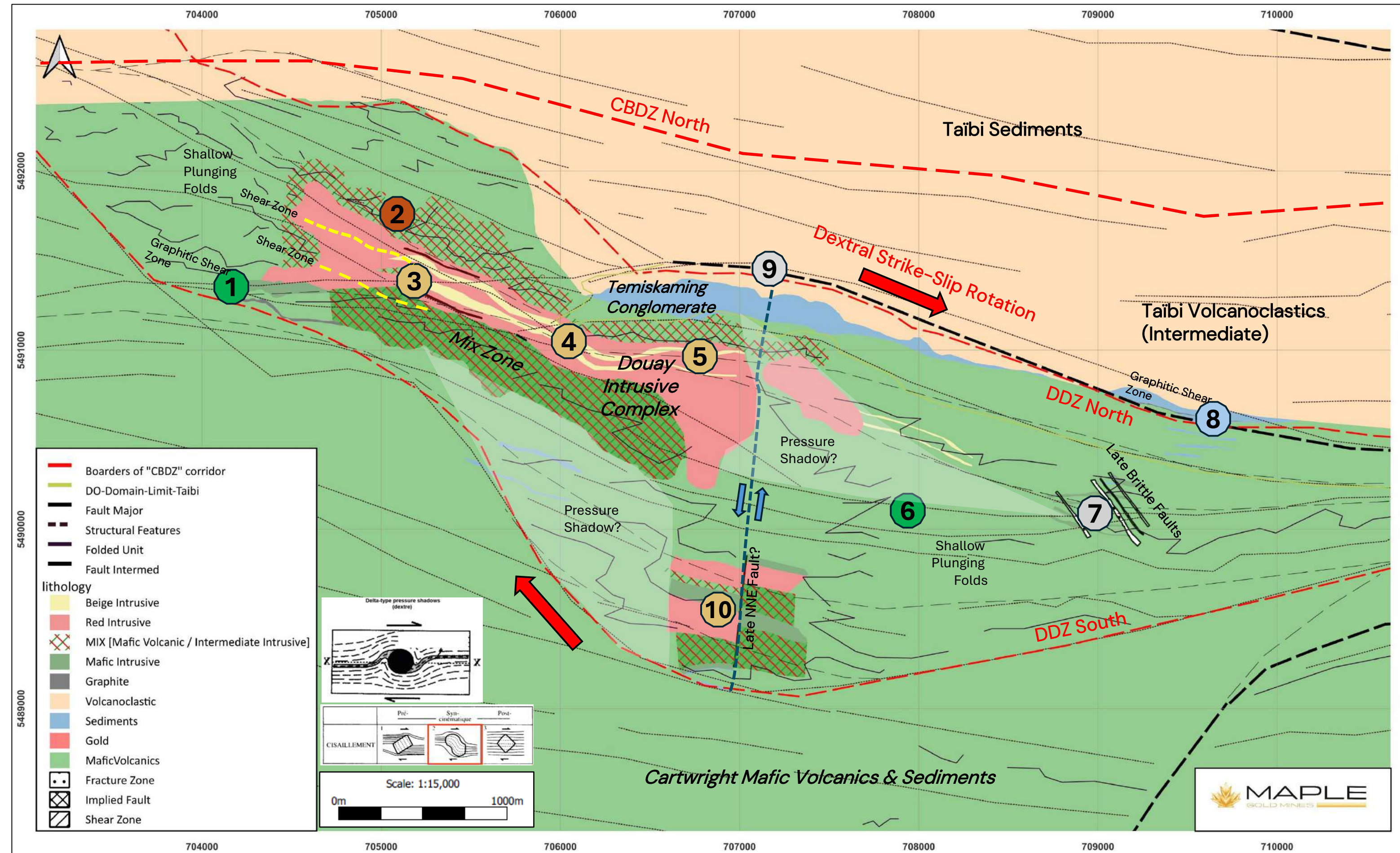
Figure: New 2024 Geology Map with preliminary targets.
