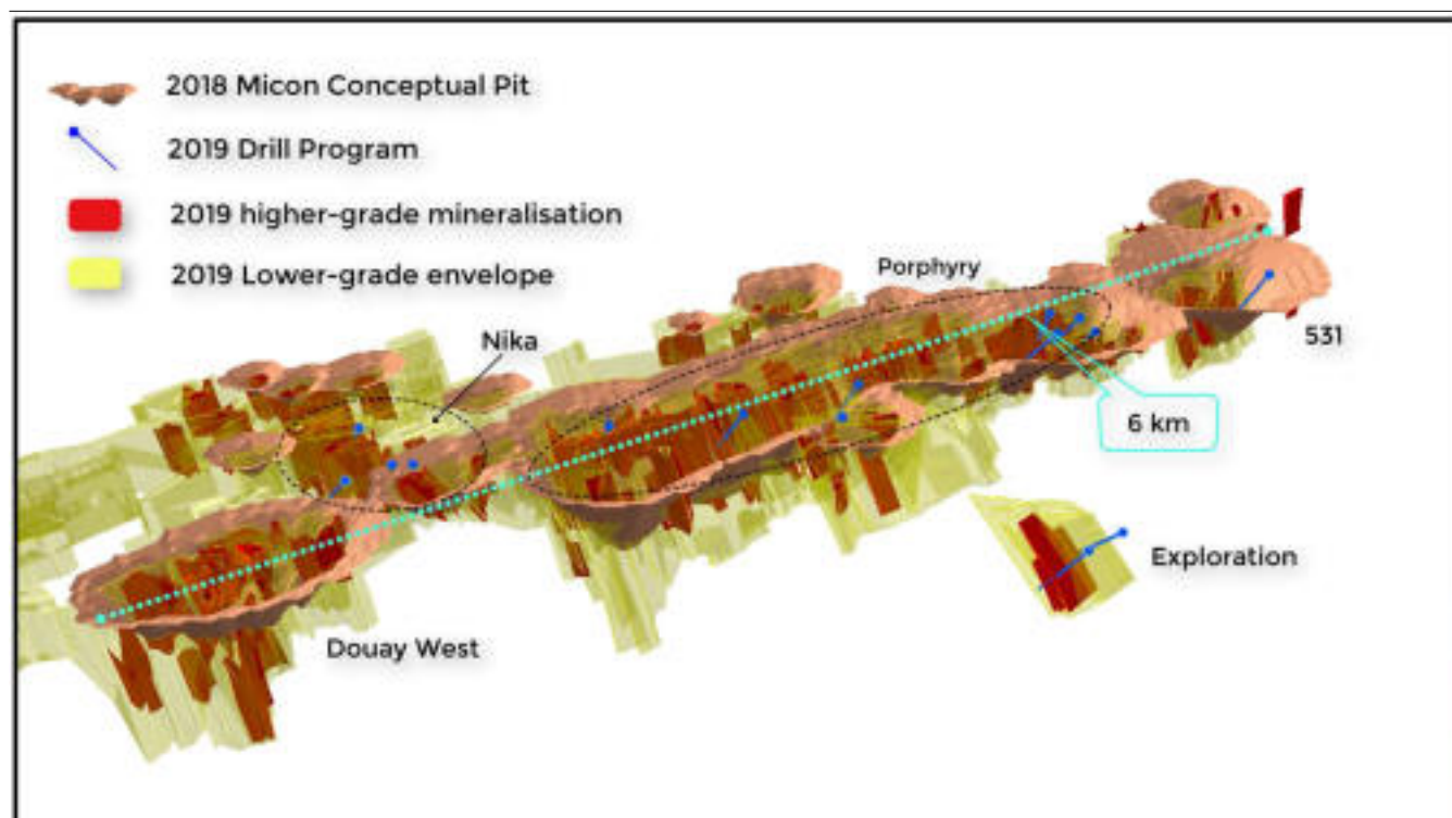
Fig. 1: Maple Gold's 3D mineralisation model with conceptual pits and distribution of drill-holes from winter 2019 program.
